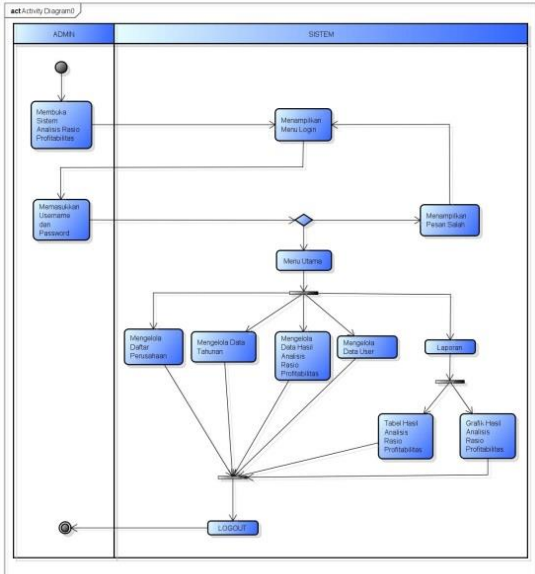
Gambar 2. Rancangan Activity Diagram Admin
