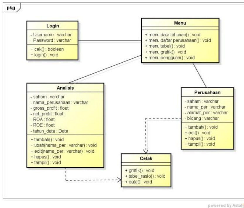
Gambar 4. Rancangan Class Diagram
