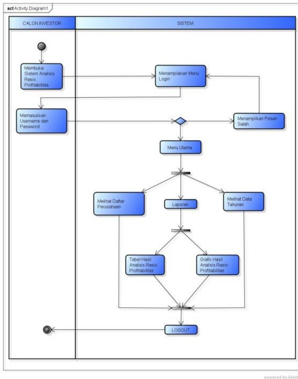
Gambar 3. Rancangan Activity Diagram Calon Investor
