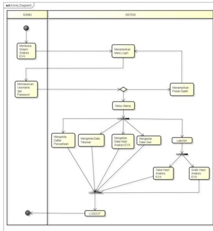
Gambar 2. Rancangan Activity Diagram Admin
