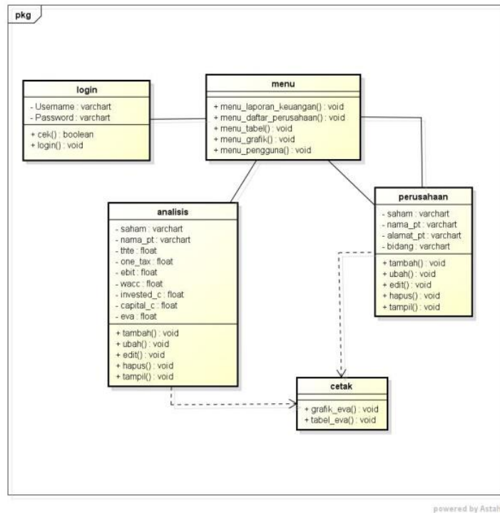
Gambar 4. Rancangan Class Diagram
